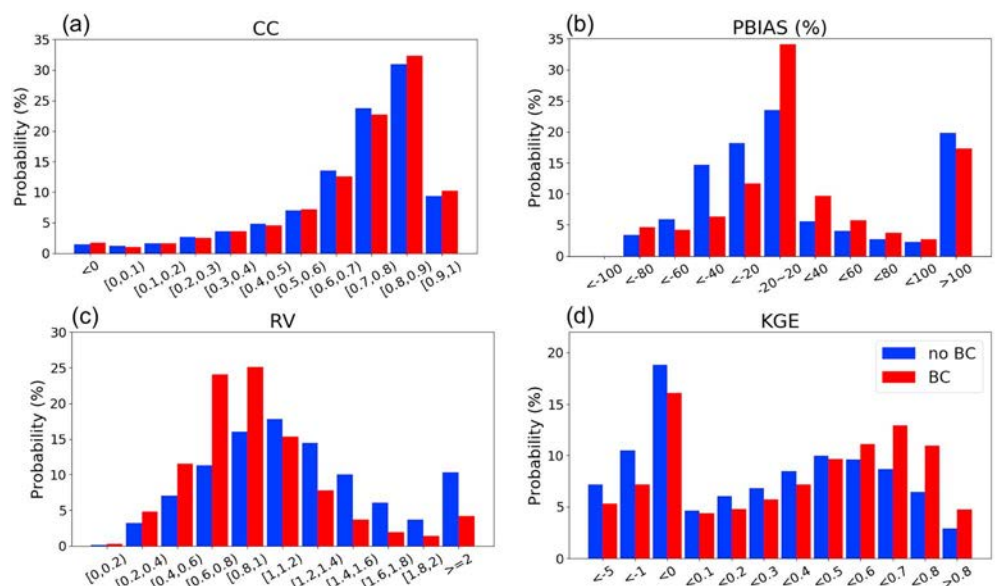
Figure 8. Histogram of the (a) CC, (b) PBIAS, (c) RV, and (d) KGE skill changes before (blue) and after BC (red bars) for the monthly simulation. CC = correlation coefficient; RV = relative variability; KGE = Kling-Gupta Efficiency; PBIAS = percentage bias; BC = bias correction.
